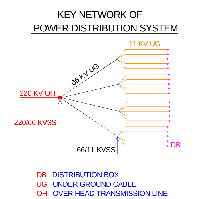
Figure 6.12: Proposed power distribution system network
